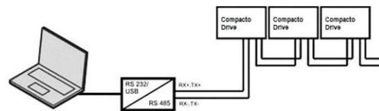
"Daisy chain" connection
